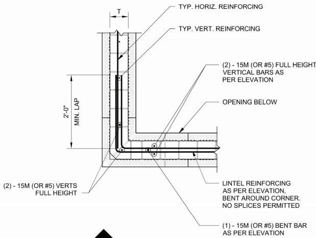
1 SECTION AT LINTEL
