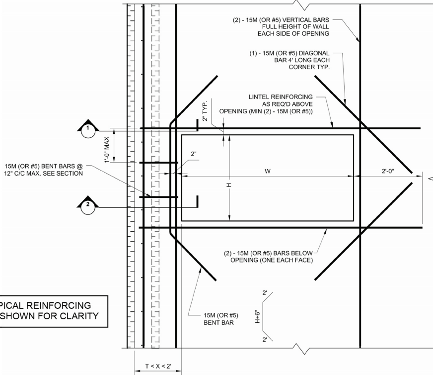
DETAIL - OPENING < 2' FROM CORNER
