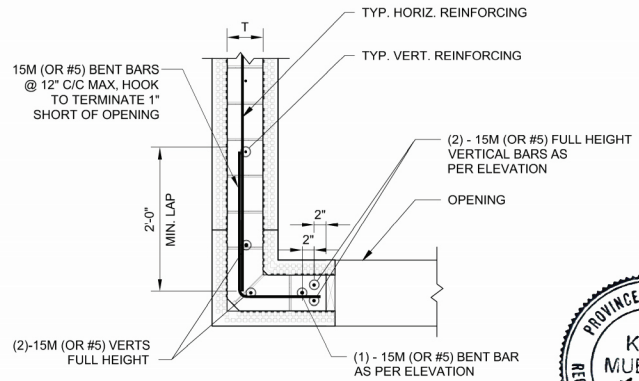
DETAIL - OPENING < 2' FROM CORNER
